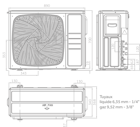
3U55S2SR5FA - 3U70S2SR5FA (3 raccords)
